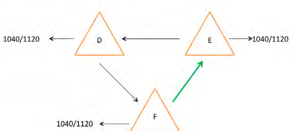
Figure A.2: Tiered and Unsolved Partnership Example
