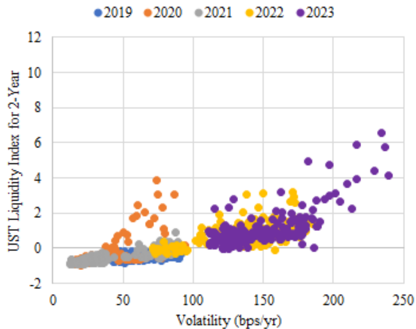
U.S. Treasury (UST) Liquidity Index* vs. Implied Volatility - 2-Year Tenor
