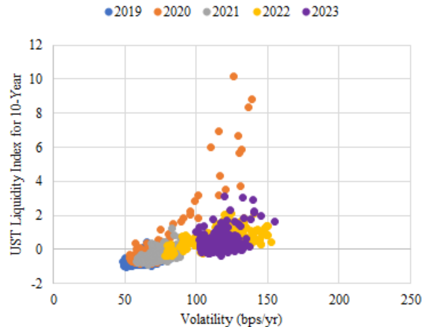
U.S. Treasury (UST) Liquidity Index* vs. Implied Volatility - 10-Year Tenor
