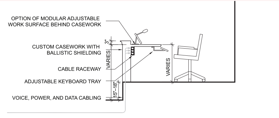
JUDGE'S BENCH PLAN + SECTION
