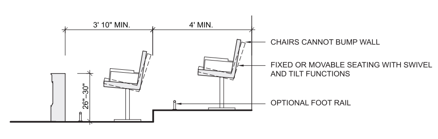
JURY BOX PLAN + SECTION
