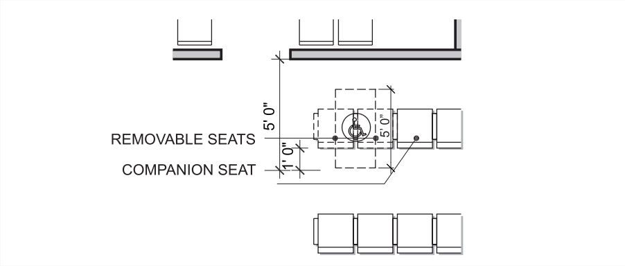
BENCH TYPE + REMOVABLE SPECTATOR SEATING
