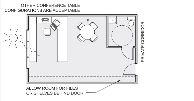
JUDGE'S CHAMBERS PLAN
